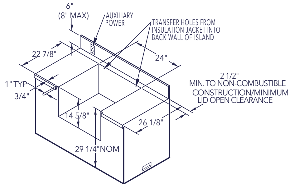
22" Caliber Pro Kamado Charcoal Grill/Smoker Insulated Jacket (CTP22IJ model) Cutout Dimensions Back Splash (No Rear Wall) Installation
