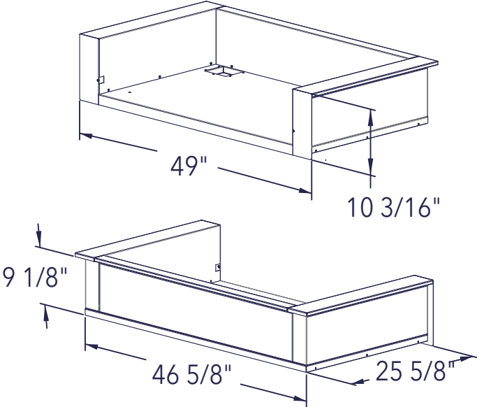
CGP42IJ 42" PRO INSULATED JACKET
