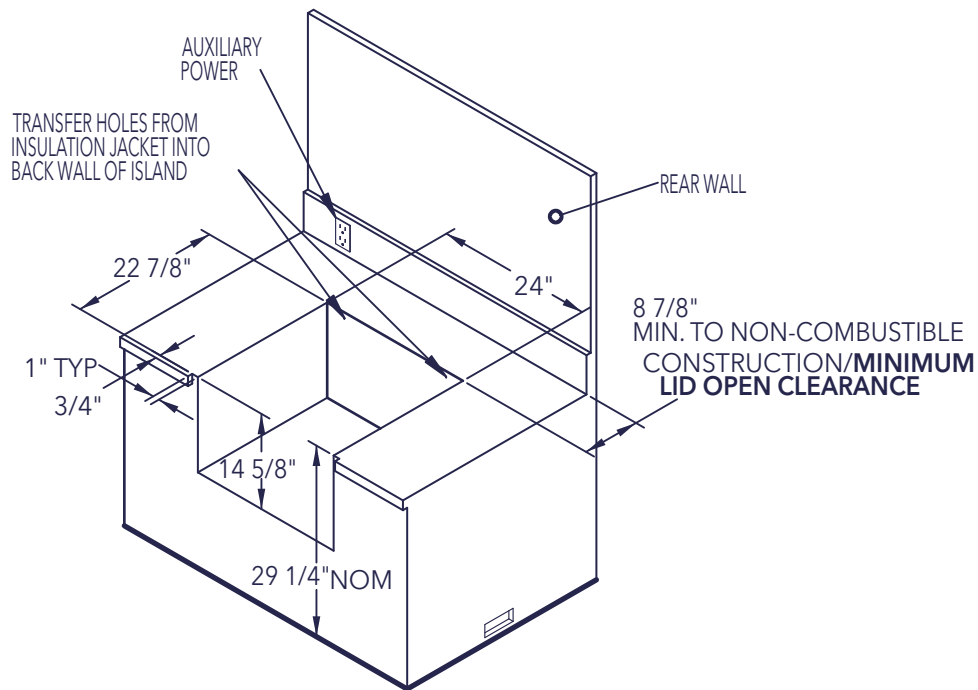
22" Caliber Pro Kamado Charcoal Grill/Smoker Insulated Jacket (CTP22IJ model) Cutout Dimensions Rear Wall Installation
