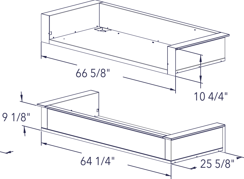
CGP60IJ 60" PRO INSULATED JACKET
