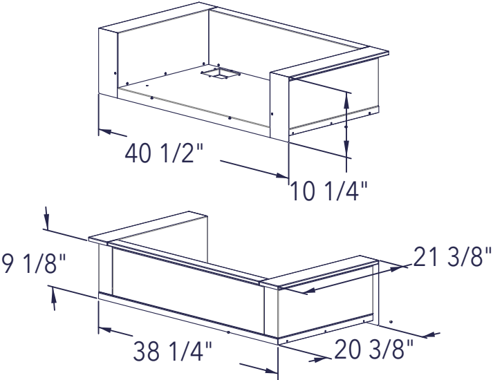
CGA35IJ 35" SILVER INSULATED JACKET
