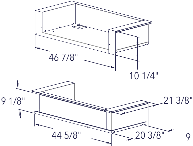
CGA41IJ 41" SILVER INSULATION JACKET
