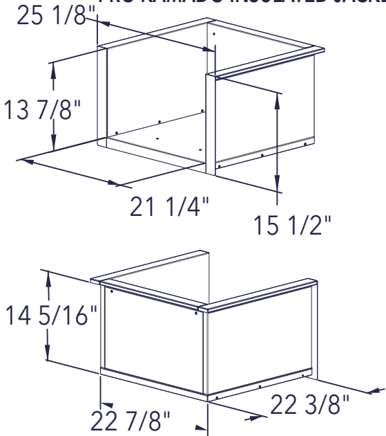
CTP22IJ PRO KAMADO INSULATED JACKET
