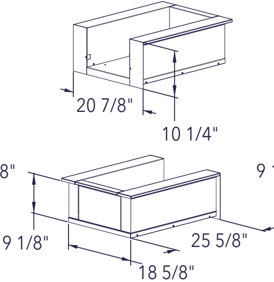
CGP14IJ DUAL SIDE BURNER INSULATED JACKET
