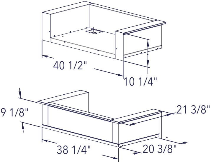
CGA35IJ 35" SILVER INSULATED JACKET
